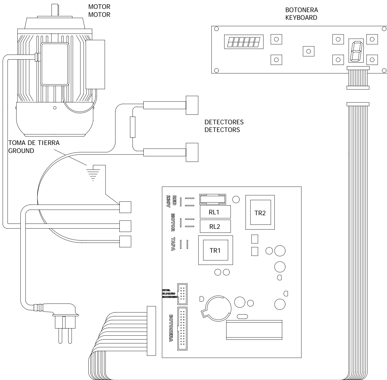
CIRCUITO DE MANIOBRA PROGRAMMING DIGITAL CIRCUIT
