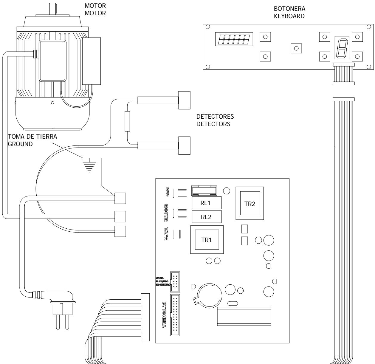
CIRCUITO DE MANIOBRA PROGRAMMING DIGITAL CIRCUIT
